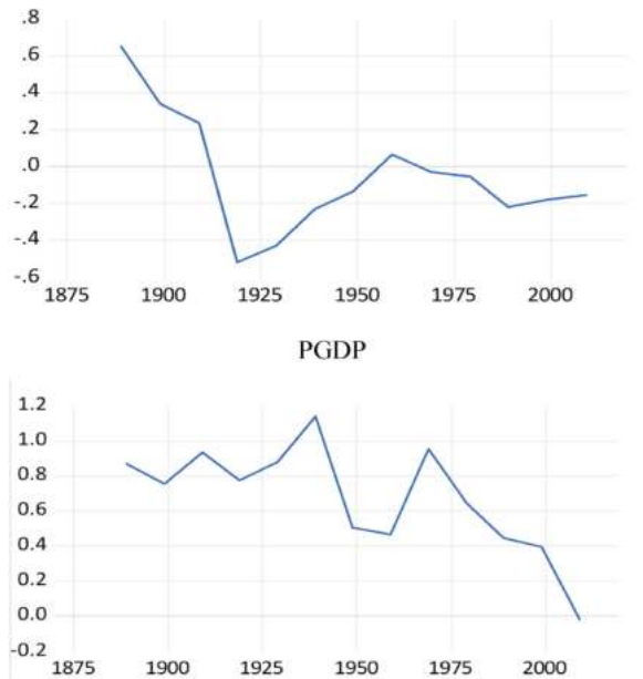
Fig. 6. Estimated coefficients from the rolling window regression for R&D and PGDP
