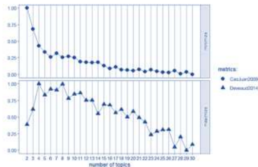
Fig. 12. Measures for selecting the optimal number of topics. Authors' calculations.
